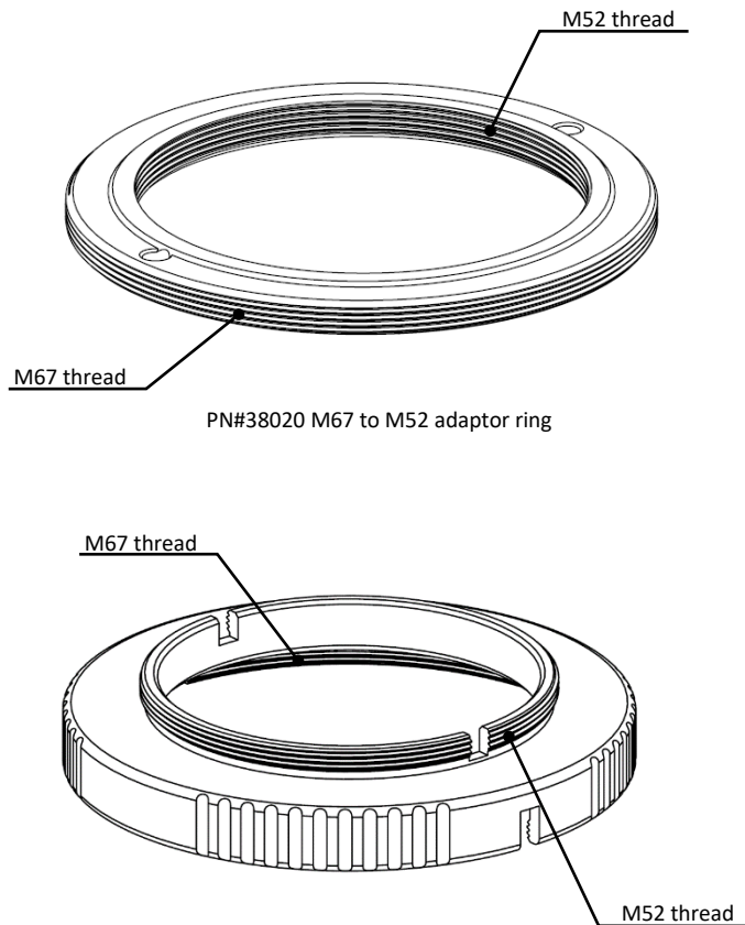
PN#38024 M52 to M67 Step Up Adaptor Ring
